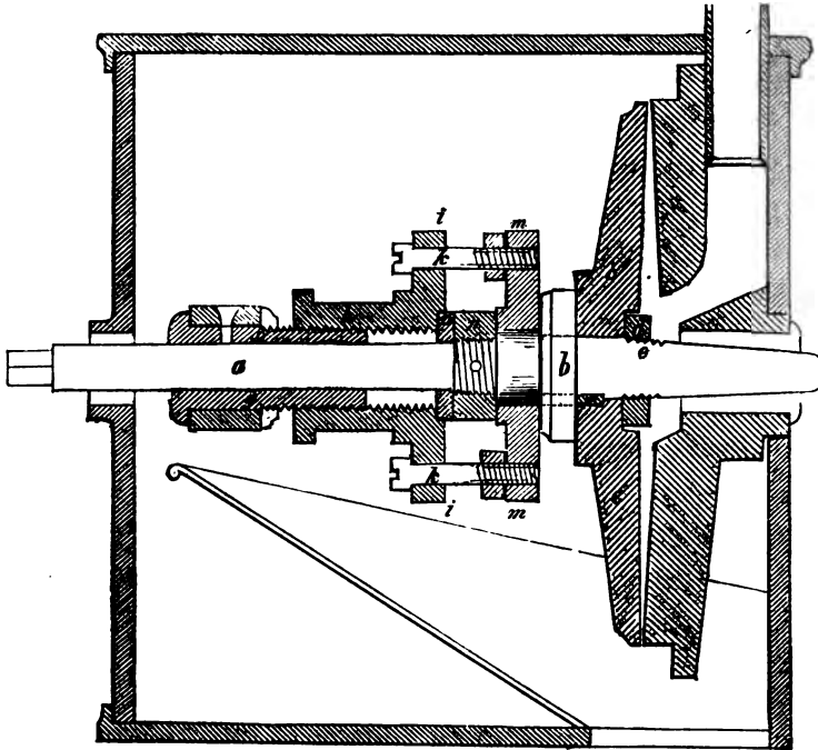
DEVERRUX'S CORN MILL.
